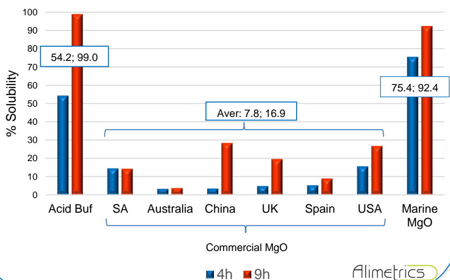
Magnesium solubility of different magnesium sources (in vitro)
